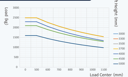
NEX Series 2.5t Load Capacity
