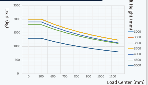
NEX Series 2.0t Load Capacity
