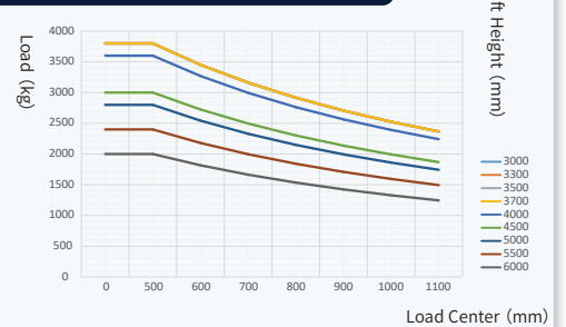
NEX Series 3.8t Load Capacity
