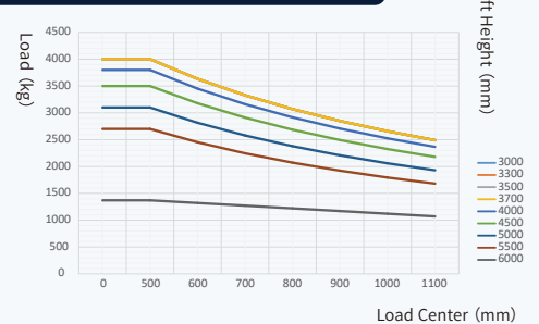
NEX Series 4.0t Load Capacity
