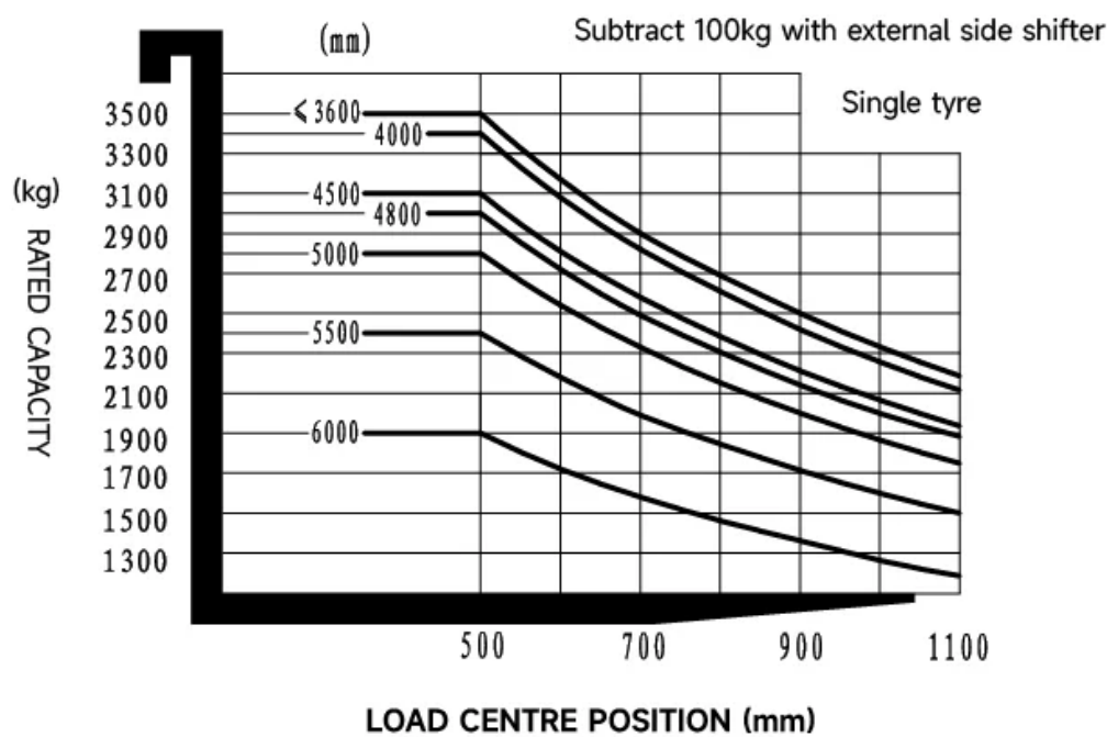
RATED CAPACITIES AND LOAD CENTERES GRAPH
